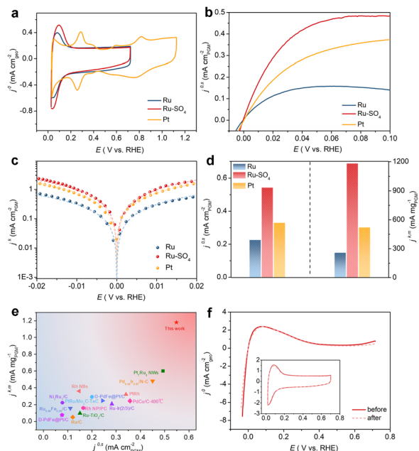
Fig. 2 (a) CV curves of Ru, Ru-SO 4 and Pt catalysts at a scanning rate of 50 mV s -1 in Ar-saturated 0.1 M KOH. (b) The HOR polarization curves of Ru, Ru-SO 4 and Pt catalysts with a scan rate of 10 mV s -1 at the rotating speed of 1600 rpm in H 2 -saturated 0.1 M KOH. (c) Tafel plots derived from HOR polarization curves of Ru, Ru-SO 4 and Pt fitted by the Butler–Volmer equation. (d) Comparison of the exchange current densities ( j^{0,s} ) and the mass activities ( j^{k,m} ) (at 50 mV) for Ru, Ru-SO 4 and Pt catalysts. (e) Comparison of j^{k,m} and j^{0,s} of Ru-SO 4 with those of noble metal-based electrocatalysts reported in the literature. Details are summarized in Table S2.† (f) The HOR polarization curves at the rotating speed of 1600 rpm in H 2 -saturated 0.1 M KOH before and after 1000 cycles. The inset figure shows the CV curves in Ar-saturated 0.1 M KOH before and after 1000 cycles.
