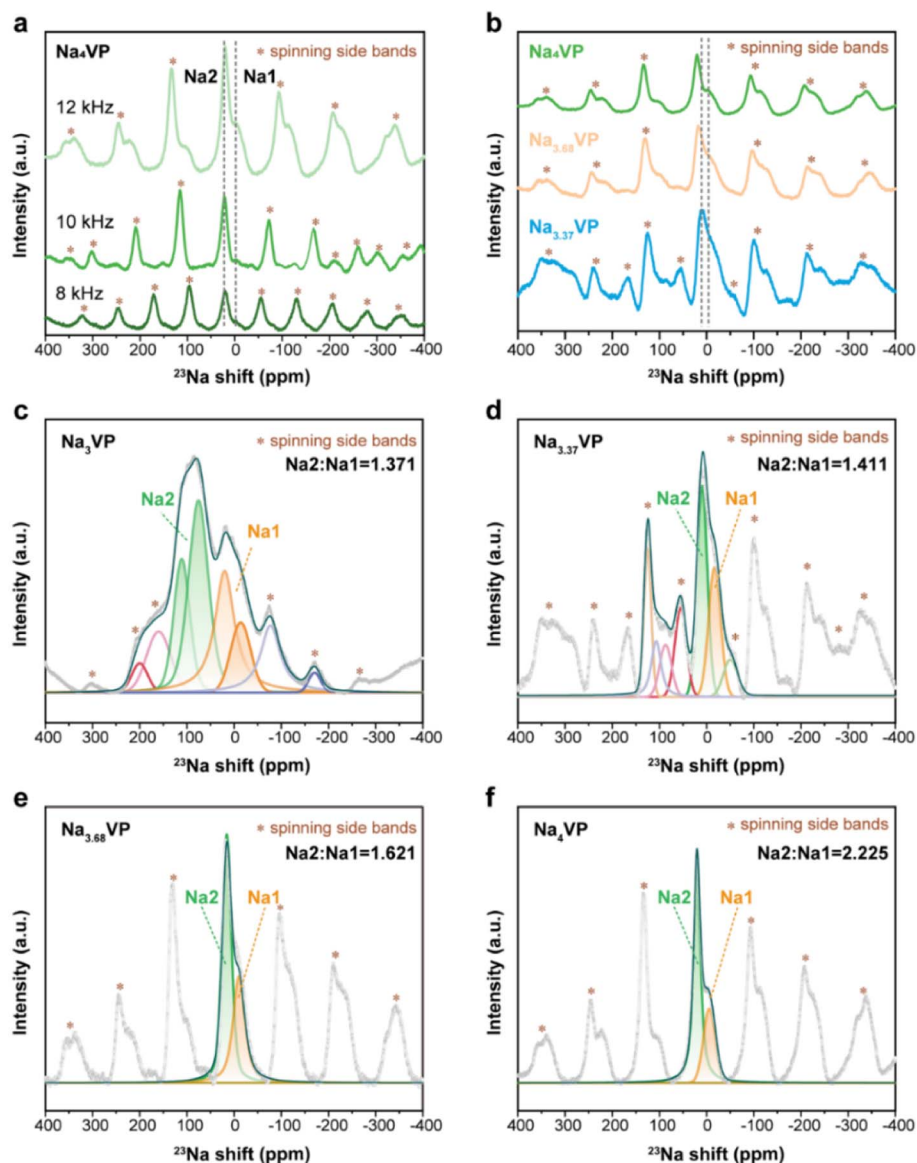
Fig. 4 (a) ^{23}\text{Na} ssNMR spectra of NaVP at 8, 10, and 12 kHz. (b) ^{23}\text{Na} ssNMR spectra of Na x VP with different sodiation depths at 12 kHz. The fitted ^{23}\text{Na} ssNMR spectra of (c) Na 3 VP, (d) Na 3.37 VP, (e) Na 3.68 VP, and (f) Na 4 VP.
