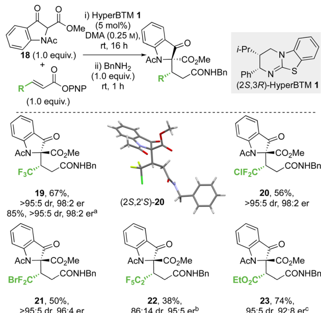
Scheme 5 Conjugate addition of methyl 1-acetyl-3-oxoindolinone-2-carboxylate to \alpha,\beta -unsaturated p -nitrophenyl esters. All products were determined by HPLC analysis on a chiral stationary phase. All product drs determined by ^1\text{H} NMR analysis of the crude reaction mixture. Following reaction conditions were applied unless stated otherwise: 0.2 mmol 18 , 0.2 mmol p -nitrophenyl ester, 0.01 mmol 1 were stirred in 0.8 mL DMA at rt for 16 h. Subsequently, 0.2 mmol \text{BnNH}_2 was added and stirred at rt for 1 h. (a) Reaction on a gram scale with purification by crystallisation. (b) 76 : 24 er of minor diastereomer, combined yield of inseparable diastereomers. (c) 72 : 18 er of minor diastereomer, combined yield of inseparable diastereomers.
