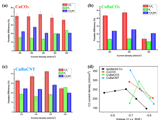
Fig. 3 Faradaic efficiency of (a) \text{CuCO}_3 , (b) \text{CuBaCO}_3 , and (c) \text{CuBaCNT} at various current densities for the \text{CO}_2\text{RR} in a flow cell. Error bars represent 1 standard deviation on the basis of three independent measurements. (d) Partial current density to C2 products (ethylene and ethanol) vs. applied potential.
