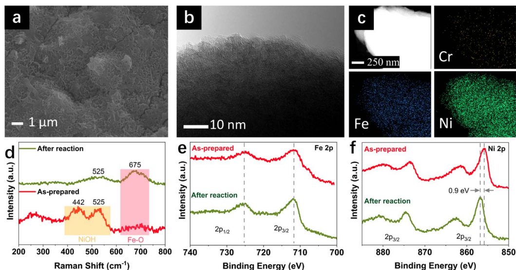
Fig. 3 Characterization of FeNiCr/FF after a three-day OER stability test at 500 \text{ mA cm}^{-2} , 50^\circ\text{C} , and 5 M KOH: (a) SEM, (b) HRTEM, (c) EDS mapping, (d) Raman spectra, and high-resolution XPS spectra for (e) Fe 2p and (f) Ni 2p.
