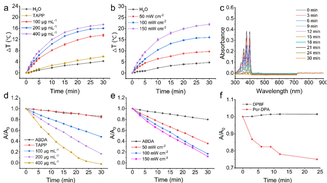
Fig. 2 (a) The time-dependent temperature changes of TAPP (200 \mu\text{g mL}^{-1} ) and Por-DPA (100, 200 and 400 \mu\text{g mL}^{-1} , respectively) when irradiated by 100 \text{mW cm}^{-2} of white light. (b) Temperature change of Por-DPA (200 \mu\text{g mL}^{-1} ) affected by irradiation power. (c) Changes of absorption spectra of ABDA with Por-DPA (400 \mu\text{g mL}^{-1} ) under 100 \text{mW cm}^{-2} of irradiation. (d) The time-dependent absorbance of ABDA at 377 nm ( A/A_0 ) without and with different concentrations of Por-DPA or TAPP (100 \mu\text{g mL}^{-1} ) under irradiation (100 \text{mW cm}^{-2} ). (e) The time-dependent absorbance (377 nm) of Por-DPA (200 \mu\text{g mL}^{-1} ) treated ABDA under different powers of irradiation. A/A_0 is the ratio of the absorbance of ABDA at a certain irradiation time to the initial absorbance of ABDA. (f) Absorbance changes of DPBF at 410 nm with pre-irradiated Por-DPA in the dark (200 \mu\text{g mL}^{-1} ).
