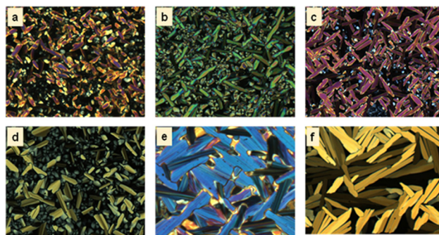
Fig. 3 POM microphotographs of the optical texture of Col phases formed by (a) P-5 at 280 ^\circ\text{C} , (b) P-6 at 230 ^\circ\text{C} , (c) P-7 at 225 ^\circ\text{C} , (d) P-8 at 190.7 ^\circ\text{C} , (e) P-10 at 150.9 ^\circ\text{C} and (f) P-11 at 214.9 ^\circ\text{C} .
