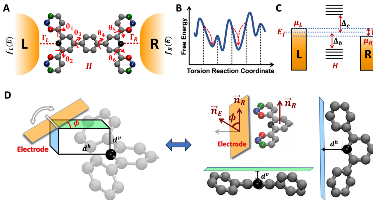
Fig. 6 Schematic of TPm molecule with six rotatable dihedrals ( \theta_1 – \theta_6 ) attached to two microscopic electrodes. In our NEGF framework (Methods subsection 5.3), H is the electronic Hamiltonian and left (L) and right (R) electrodes are implicitly modeled in terms of their Fermi functions ( f_{L/R} ) and coupling to the molecule \Gamma_{L/R} . (B) Schematic conformational energy landscape with initial set of enumerated conformations shown by vertical dotted lines. Upon geometry optimization, each such conformation relaxes to a local minimum (red arrows). (C) Schematic energy level diagram showing the electron/hole transport barriers ( \Delta_e/\Delta_h ) governing the charge transport across a molecular junction. The electrode electronic levels are governed by Fermi statistics and expressed in terms of the chemical potentials of left ( \mu_L ) and right ( \mu_R ) electrodes and their Fermi level ( E_f ). (D) Model for electrode–pyridyl attachment to calculate the screening distance ( d_{\text{eff}} ) for linking N-atoms that are not directly accessible to electrodes. The angle \phi describes the tilt of the electrode plane relative to the plane of the pyridyl ring containing the N-atom of interest. Two extremes of the electrode approach (at \phi = 0 and \pi/2 ) to the core N-atom where d_{\text{eff}} = d^v and d_{\text{eff}} = d^h .
