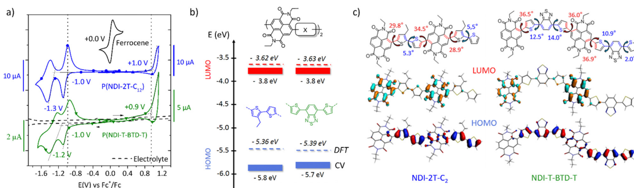
Fig. 3 (a) Cyclic voltammograms of both NDI-based copolymers. Experimental conditions: acetonitrile (MeCN), scan rate = 50 \text{ mV s}^{-1} , 0.1 \text{ M} [NBu 4 ][PF 6 ], Pt electrode, 0.01 \text{ M} Ag/AgNO 3 calibrated Fc + /Fc. (b) Comparison of CV-measured (thick lines \pm 0.1 \text{ eV} ) and DFT-calculated (dashed lines) HOMO and LUMO energy levels. (c) Ground-state DFT calculations: (top) geometry-optimized structures and dihedral angles (VWN + PBE/TZ2P/Grimme 3/MeCN), (middle and bottom) LUMO and HOMO electronic density distributions, respectively (B3LYP/TZ2P/MeCN). The copolymers are approximated to dimers and the alkyl chains are replaced by ethyl chains.
