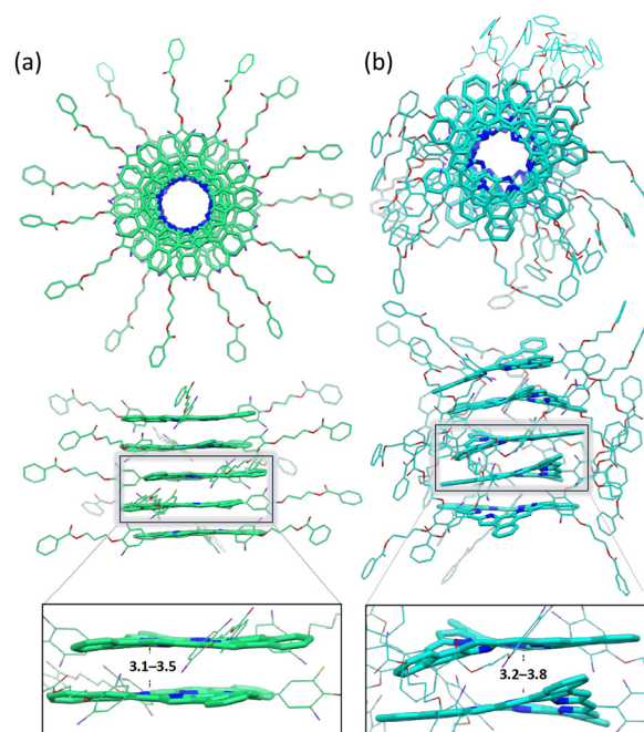
Fig. 3 Top and side views of the supramolecular pentamers of (a) NRos-2 and (b) NRos-3 fully optimized at the GFN2-xTB level. Carbons atoms of NRos-2 and NRos-3 are represented in green and blue, respectively.
