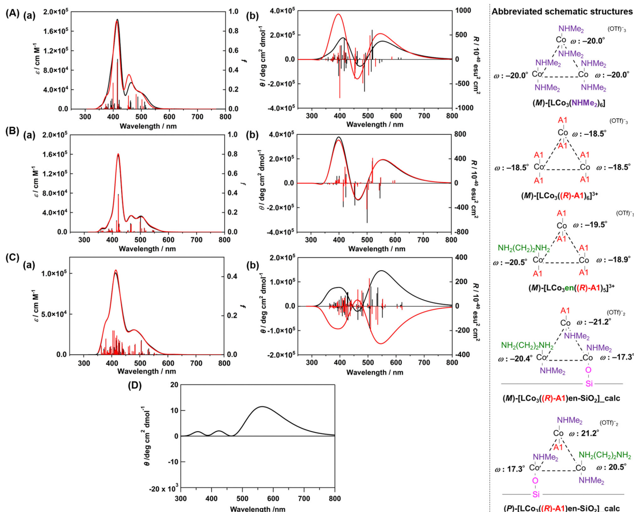
Fig. 2 (A) Calculated (a) UV-vis and (b) CD spectra of (M)\text{-}[\text{LCo}_3(\text{NHMe}_2)_6]^{3+} (black) and (M)\text{-}[\text{LCo}_3((R)\text{-A1})_6]^{3+} (red) (in acetonitrile). (B) Calculated (a) UV-vis and (b) CD spectra of (M)\text{-}[\text{LCo}_3((R)\text{-A1})_6]^{3+} (black) and (M)\text{-}[\text{LCo}_3\text{en}((R)\text{-A1})_5]^{3+} (red) (in vacuum). (C) Calculated (a) UV-vis and (b) CD spectra of the modelled structure of \text{LCo}_3((R)\text{-A1})/\text{en-SiO}_2_{\text{calc}} ( M configuration) (black) and \text{LCo}_3((R)\text{-A1})/\text{en-SiO}_2_{\text{calc}} ( P configuration) (red) (in vacuum). (D) The summed simulated CD spectrum of the modelled structure of \text{LCo}_3((R)\text{-A1})/\text{en-SiO}_2_{\text{calc}} ( M configuration) and \text{LCo}_3((R)\text{-A1})/\text{en-SiO}_2_{\text{calc}} ( P configuration) with the ratio of 55/45. Abbreviated schematic structures (see ESI† and Fig. S2 for details) of the optimized trinuclear cobalt complexes are also presented. The torsion angles of each saloph moiety of the optimized structures under vacuum are also shown as \omega .
