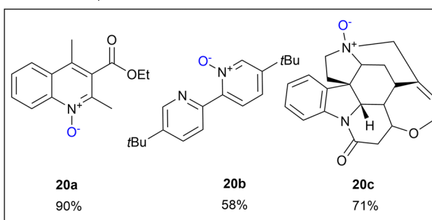
Scheme 6 N-Oxidation with peroxodisulfate. * Ethanol is used as a co-solvent.
