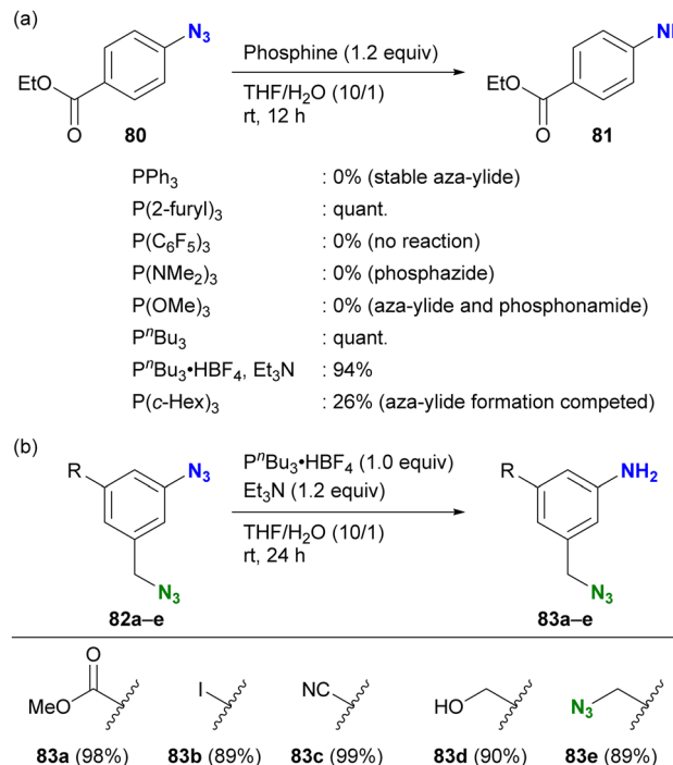
Scheme 16 Aryl azide-selective Staudinger reduction (a) scope of phosphines without formation of aza-ylides (b) application to the di- and triazide substrates.
