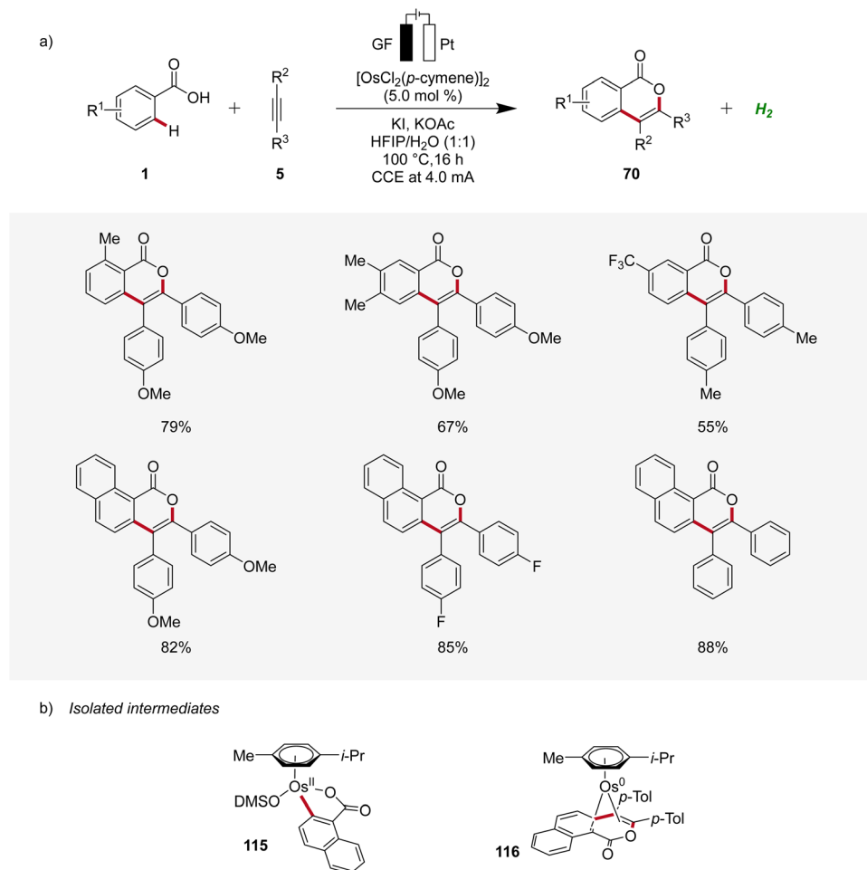
Scheme 34 Osmoelectro-catalyzed alkyne annulation by weakly coordinating acids 1 .
