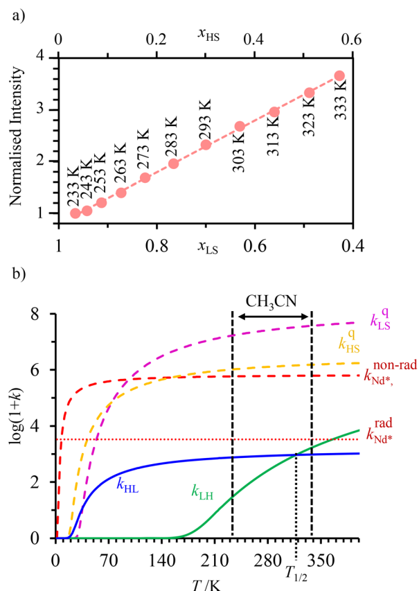
Fig. 10 (a) Steady-state \text{Nd}(\text{F}_{3/2}) NIR luminescence monitoring of the \text{Fe}(\text{II}) spin-state in the dinuclear [\text{Fe}(\text{II})\text{Nd}(\text{L10})_3]^{5+} helicate in acetonitrile ( x_{\text{LS}} = 1 - x_{\text{HS}} is the mole fraction of low-spin \text{Fe}(\text{II}) ) and (b) associated kinetic rate constants (see Fig. 8 for the kinetic scheme). This figure has been adapted from ref. 77 with permission from American Chemical Society, copyright 2024.
