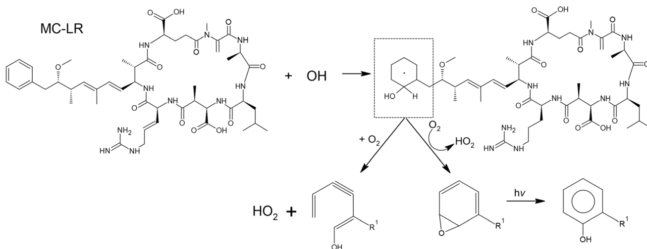
Scheme 3 Reaction of •OH on the aromatic ring of MC-LR.
