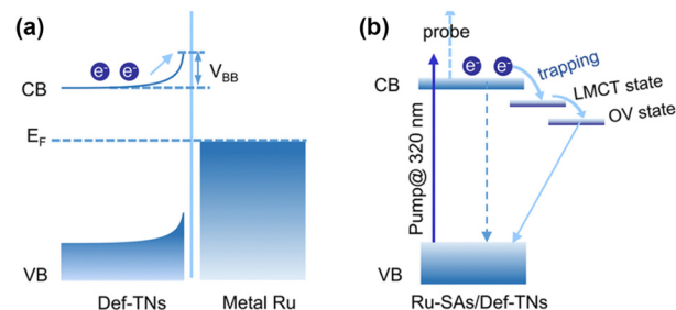
Fig. 5 Mechanisms underlying the photoexcited electron dynamics involved in (a) Ru-NPs/Def-TNs and (b) Ru-SAs/Def-TNs. Reprinted with permission from ref. 83. Copyright 2020 American Chemical Society.
