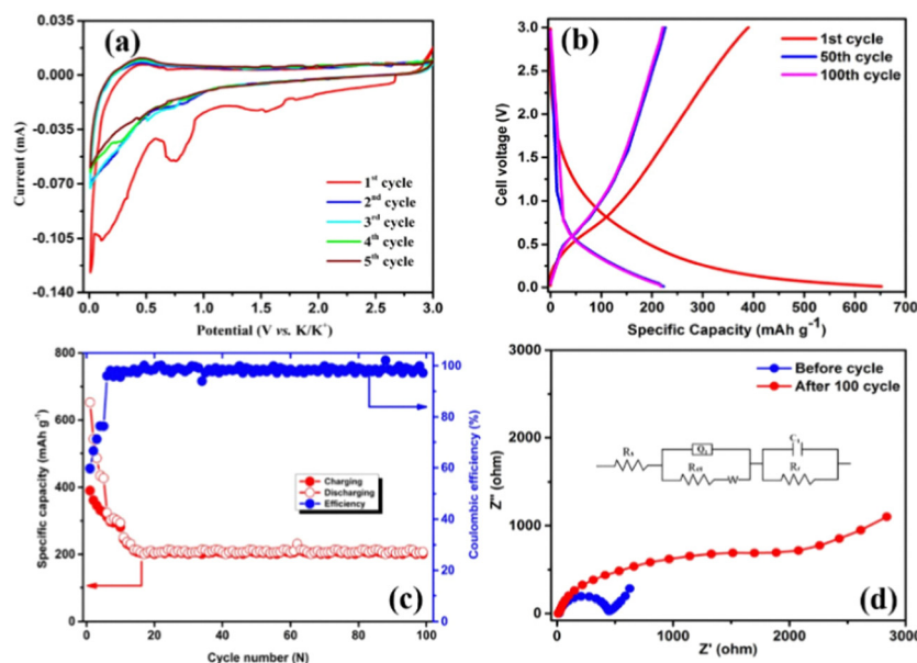
Fig. 6 (a) Cyclic voltammogram of the synthesized AGC anode cycled between 0.1 and 3.0 V vs. K + /K with the scan rate of 0.05 mV s -1 . (b) Discharge-charge profiles of the AGC anode at 100 mA g -1 . (c) Cycling stability and coulombic efficiency of the AGC anode at the current density of 100 mA g -1 . (d) EIS spectra of the as-fabricated AGC anode (blue color) and the cell under the influence of 100 mA g -1 after 100 cycles (red color) and the fitted equivalent circuit.
