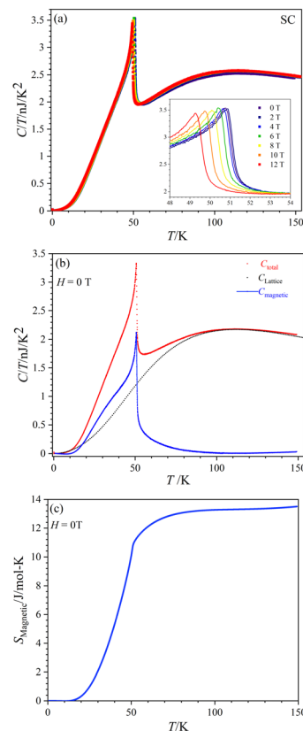
Fig. 8 (a) C/T vs. T curves of CoTeO 4 in the range 0 \leq H \leq 12 T. Inset in (a) represents the zoom view of peak maxima. (b) Magnetic (blue) and lattice (black) contributions of C/T vs. T for H = 0 T. (c) S magnetic vs. T for H = 0 T.
