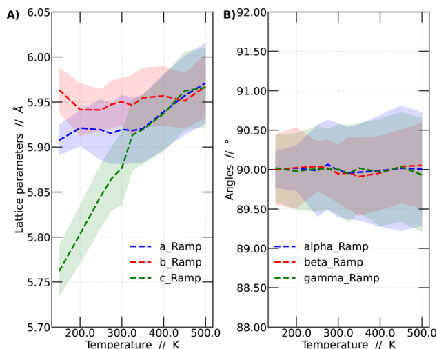
Fig. 2 (A) Variation of the average lattice parameters ( a , b and c ) and (B) angles among lattice vectors (alpha, beta and gamma) as a function of temperature for CsPbBr 3 . The standard deviation (STD) is depicted using a shaded region.
