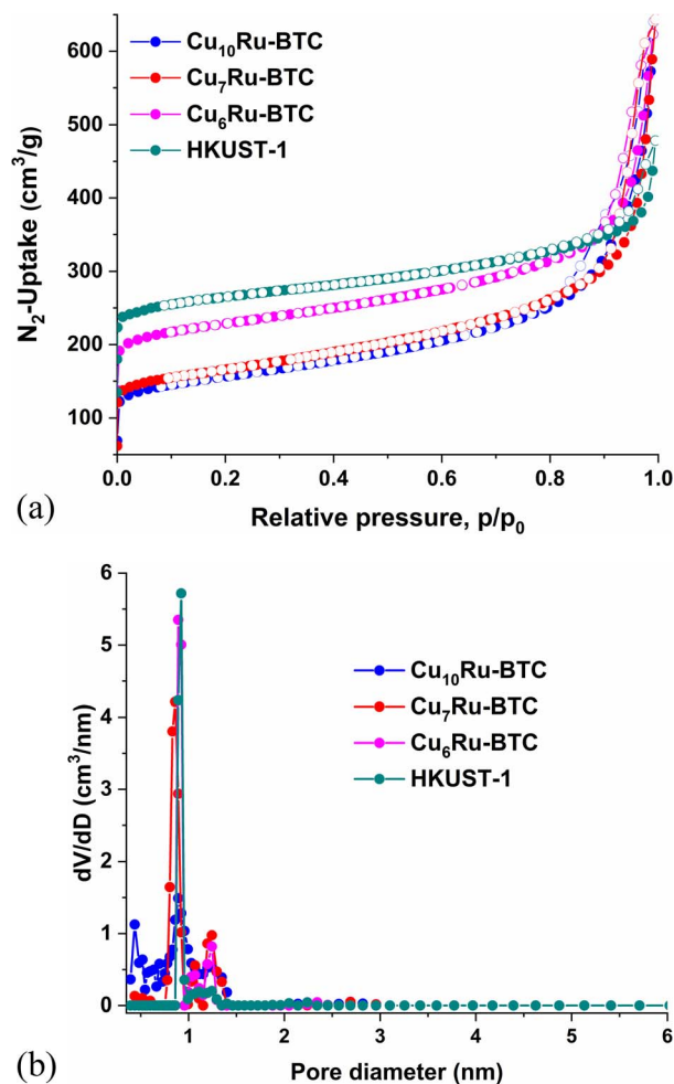
Fig. 4 (a) \text{N}_2 -sorption isotherms at 77 \text{ K} (adsorption filled circles; desorption empty circles) and (b) NLDFT-derived pore size distributions of \text{Cu}_6\text{Ru-BTC} , \text{Cu}_7\text{Ru-BTC} , \text{Cu}_{10}\text{Ru-BTC} and mechanochemically synthesized HKUST-1 (model cylindrical pores at metal oxide).
