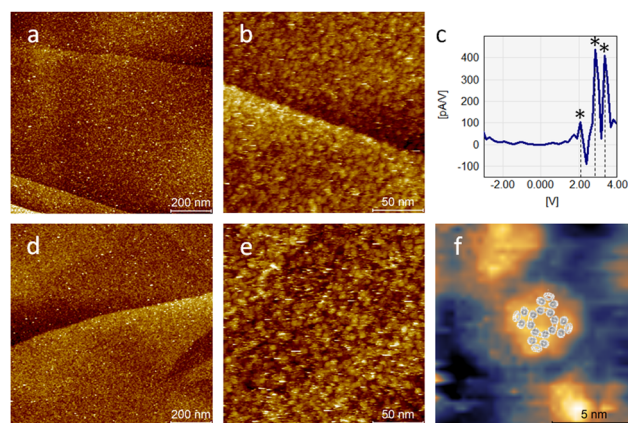
Fig. 3 STM images ( U_B = 2 V; I_T = 10 pA) of a (\text{PcDy})_2\text{-POV12} layer (a) and (b) with corresponding dI/dV curve (c) measured on a single point in (b) and of a \text{PcDyOAc} layer (d) and (e). High resolution imaging of a single \text{PcDyOAc} molecule (f) exhibits Pc characteristic fourfold symmetry indicated by the overlay of a calculated metal Pc LUMO structure. 43
