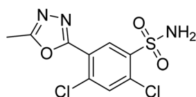
2,4-Dichloro-5-(5-methyl-1,3,4-oxadiazol-2-yl)benzenesulfonamide
