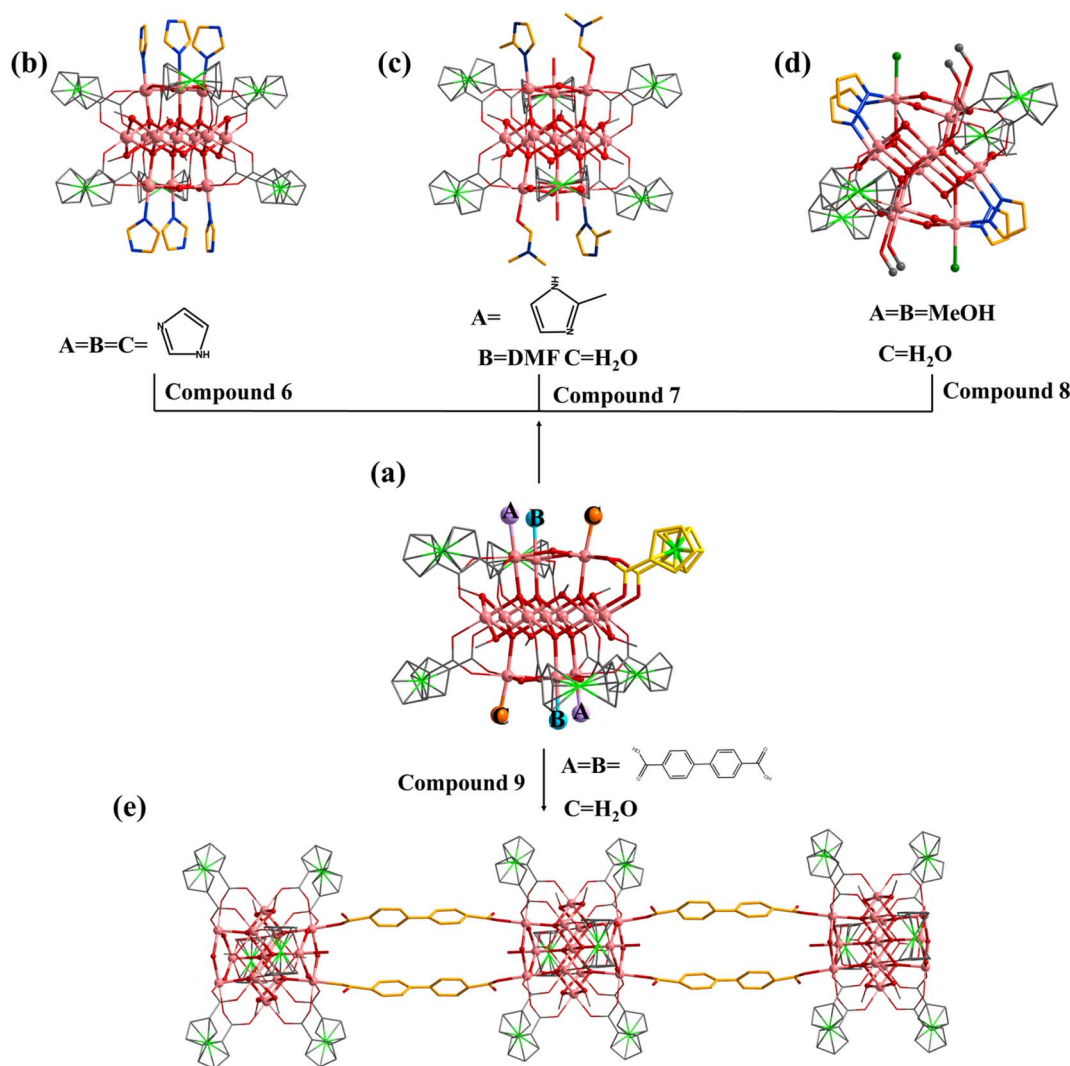
Fig. 5 (a) [\text{In}_{13}] as a secondary building unit; (b) compound 6 ( A = B = C = \text{HIm} ); (c) compound 7 ( A = 2\text{-mim} , B = \text{DMF} , C = =\text{H}_2\text{O} ); (d) compound 8 ( A = B = \text{MeOH} , C = =\text{H}_2\text{O} ); (e) compound 9 ( A = B = \text{BPDC} , C = =\text{H}_2\text{O} ). A, B and C represent different substitution sites.
