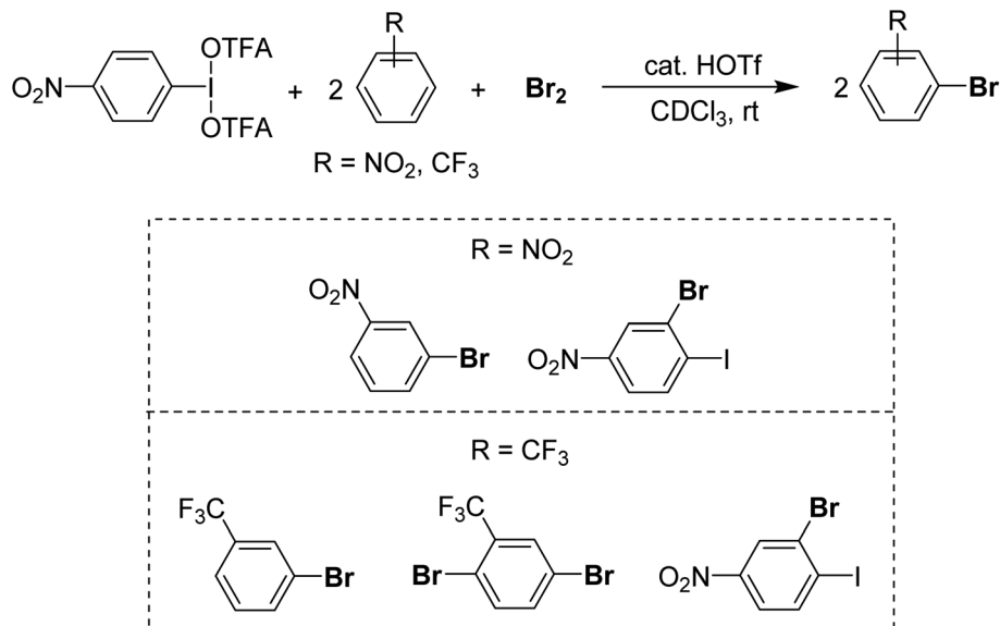
Scheme 21 Activation of \text{Br}_2 and \text{Br}^- via \text{I}(\text{III}) resulting in delivery of two equivalents of \text{Br} to an electron-poor substrate.
