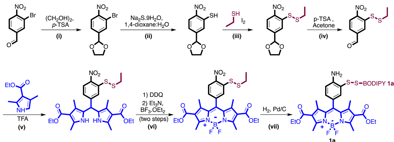
Scheme 1 The synthesis of probe 1a with 2-aminothiophenol reactive core and BODIPY for fluorescence. (i) Toluene, 60^\circ\text{C} , 6 h, 97%; (ii) 1,4-dioxane, water (2 : 1), 0^\circ\text{C} \rightarrow \text{rt} , 20 h, 75%; (iii) DMSO, 50^\circ\text{C} , 7 h, 76%; (iv) acetone, reflux, 7 h, 56%; (v) DCM, rt, 5 h, 92%; (vi) DCM, 0^\circ\text{C} \rightarrow \text{rt} , 5 h, 72%; (vii) DCM, rt, 5 h, 46%.
