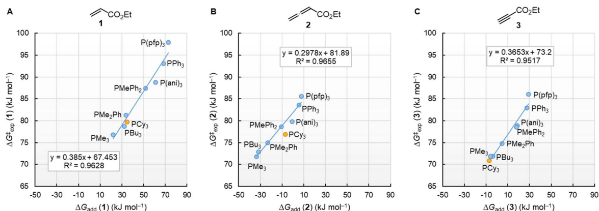
Fig. 12 Correlations of \Delta G^\ddagger_{\text{exp}} (20 °C) for \text{PR}_3 additions to (A) 1 , (B) 2 , and (C) 3 in dichloromethane with the respective reaction energies \Delta G_{\text{add}} . With energies from Table 4, data for the sterically encumbered \text{PCy}_3 excluded when constructing the correlation lines.
