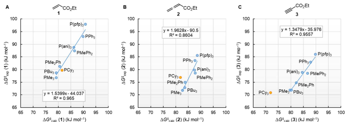
Fig. 13 Correlation of experimentally determined \Delta G^\ddagger_{\text{exp}} (20 °C) for \text{PR}_3 additions to (A) 1 , (B) 2 , and (C) 3 in dichloromethane with quantum-chemically calculated Gibbs activation energies ( \Delta G^\ddagger_{\text{calc}} ). Results for \text{PCy}_3 were excluded when calculating the regression lines.
