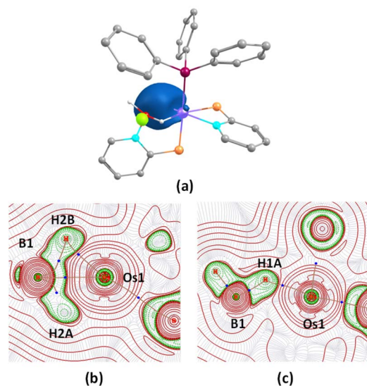
Fig. 8 (a) 3c–2e bonding interaction along the Os–H–B plane in 5' (isovalue 0.004 [ e \text{ bohr}^{-3} ] 1/2 ); (b) and (c) contour-line diagram of the Laplacian of the electron density along the Os–H–B planes in 5' and trans - 6 , respectively.
