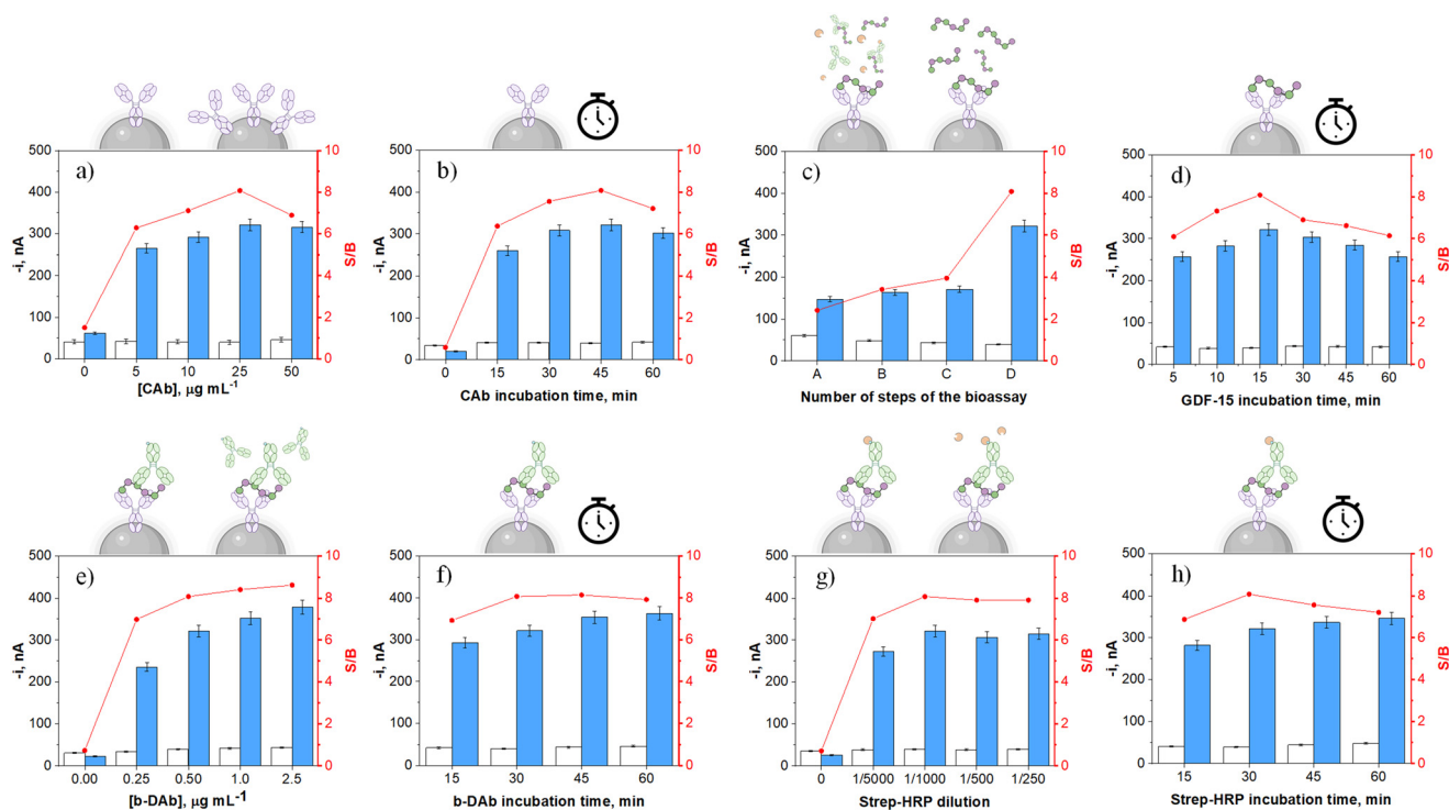
Fig. 1 Dependence of the amperometric responses obtained with the developed immunoplatform in the absence (B, white bars) and in the presence (S, blue bars) of 1000 \mu\text{g mL}^{-1} GDF-15, concerning the following variables: (a) CAB concentration and (b) incubation time, (c) number of steps involved in the assay (see main text for A–D symbols meaning), (d) target GDF-15 incubation time, (e) b-DAB concentration and (f) incubation time, (g) strep-HRP conjugate dilution, and (h) incubation time. The resulting S/B ratios are represented by red dots and lines.
