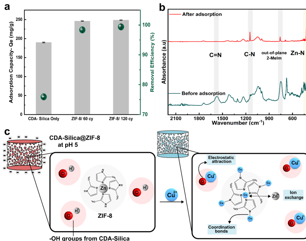
Fig. 5 Heavy metal removal: (a) adsorption capacity ( mg\ g^{-1} ) and removal efficiency (green circles, %) for 20 mg of the adsorbent (aerogel) load in 100\ mg\ L^{-1} of stock solution of Cu^{2+} ions and (b) FTIR spectra of CDA-silica@ZIF-8/120cy before and after adsorption of Cu^{2+} . Note that all three samples in (a) are aerogels. (c) Adsorption mechanism depicting ion-exchange with Zn, formation of coordination complex of Cu with N atoms of ZIF-8, and electrostatic interactions between hydroxyl groups of CDA-silica and Cu.
