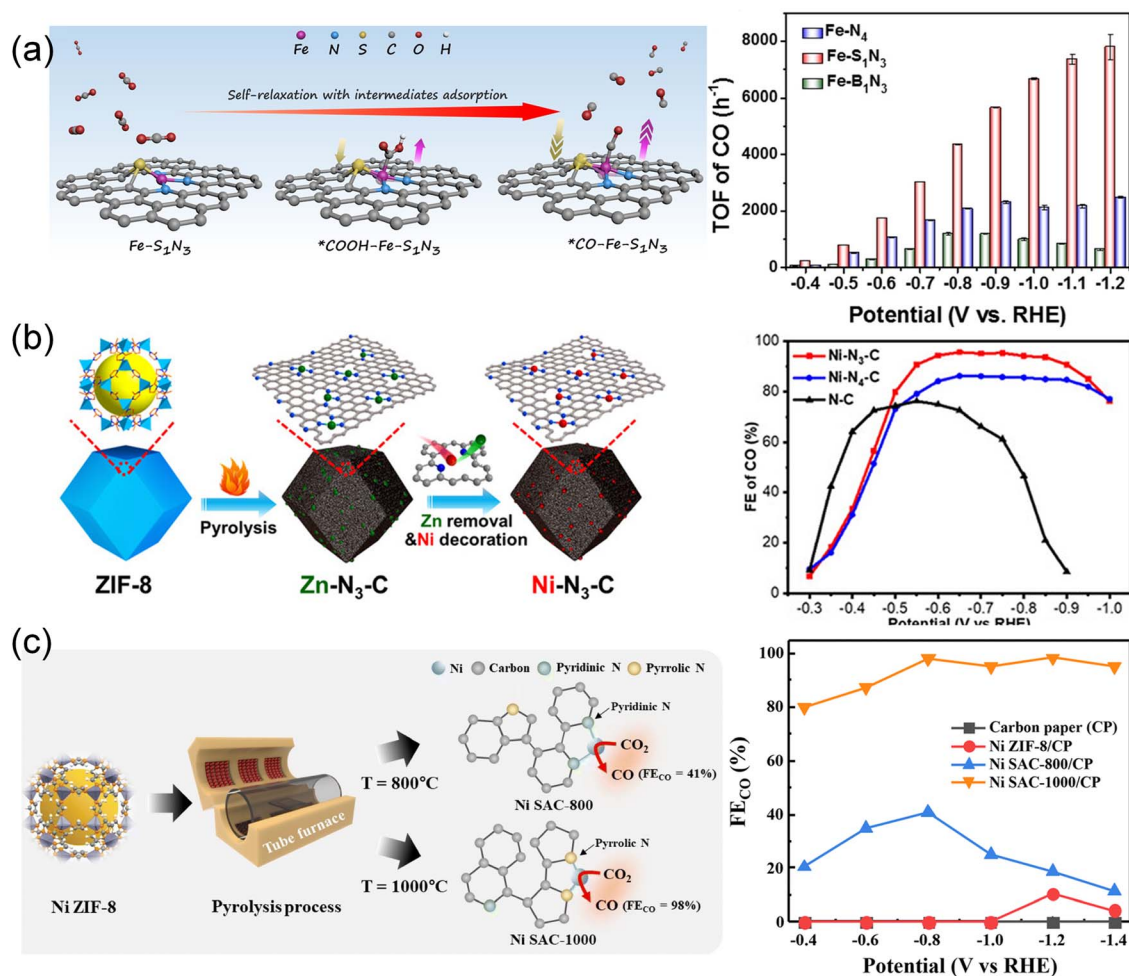
Fig. 10 (a) Schematic illustration showcasing the structural distortion of the \text{Fe-S}_1\text{N}_3 site with various adsorbed intermediates. 47 Copyright 2023, Wiley-VCH. (b) Schematic illustration for the fabrication of low-coordination single-atom Ni electrocatalysts. 48 Copyright 2021, Wiley-VCH. (c) Schematic illustration for the fabrication of pyrrolic N-stabilized low-coordinated Ni SAC and \text{FE}_{\text{CO}} at different potentials. 89 Copyright 2024, Royal Society of Chemistry.
