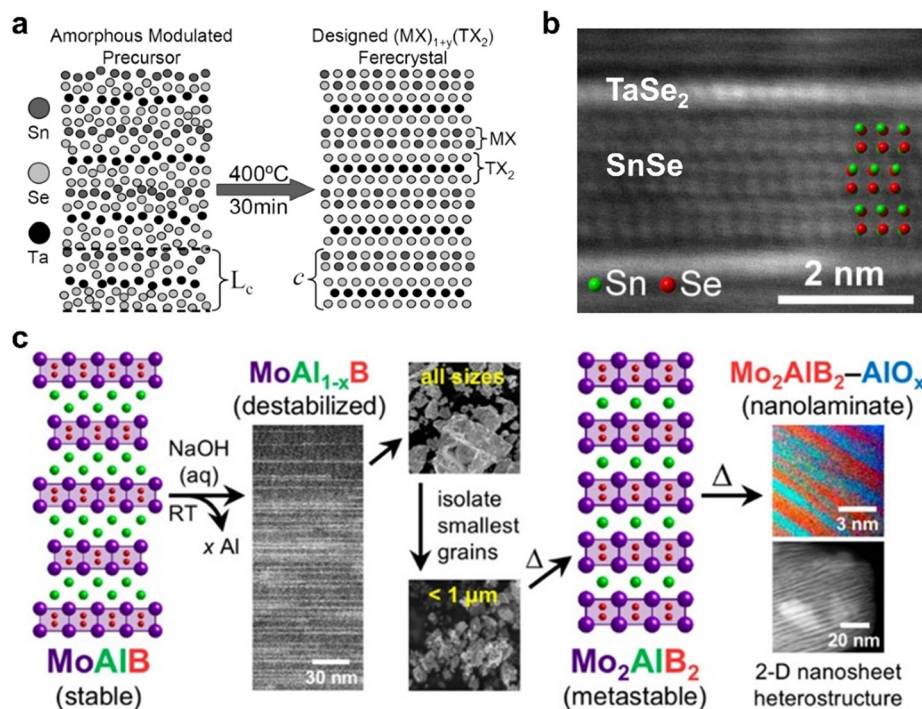
Fig. 4 (a) Schematic of an as-deposited amorphous precursor on the left, and [(SnSe) 1.15 ] 1 (TaSe 2 ) 1 which forms after annealing on the right; (b) cross-sectional high-resolution high angle annular dark field scanning transmission electron microscopy (HAADF-STEM) image of a [(SnSe) 1.15 ] 1 (TaSe 2 ) 1 specimen, with layers noted and Sn and Se indicated with green and red beads, respectively; (c) scheme depicting the topotactic conversion of MoAlB to MoAl 1-x B, followed by isolation of smaller grains and thermal annealing to achieve metastable Mo 2 AlB 2 and finally a 2D nanosheet heterostructure composed of alternating Mo 2 AlB 2 and AlO x layers of 1–3 nm thickness. Panels (a) and (b) are adapted with permission from The American Chemical Society, 103 and panel (c) is reprinted with permission from The American Chemical Society. 105
