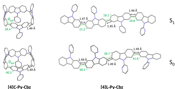
Fig. 5 Optimized geometries (B3LYP/6-31+g(d)) S_0 (ground state, bottom) and S_1 (first singlet excited state, top) of [4]C-Py-Cbz (left) and [4]L-Py-Cbz (right). On each structure, in the S_0 and S_1 states, the modeled mean torsion angle \theta_{\text{ext}} between the carbazoles and the length of the C-C bond linking two carbazoles are presented.
