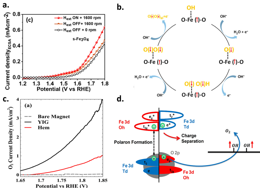
Fig. 15 Triplet pathway of water oxidation via spin-polarized hole accumulation on magnetic catalysts. (a) Influence of stirring and external magnetic field ( H_{\text{ext}} ) on \text{s-Fe}_3\text{O}_4 . (b) Spin-selective OER mechanism under a magnetic field. (c) \text{O}_2 current density for pristine magnetic electrodes, hematite, and YIG. (d) Schematic of the formation of polarons and electron-hole recombination at Oh sites, resulting in spin-polarized hole accumulation on the YIG surface, which facilitates triplet-pathway water oxidation and \text{O}_2 generation. Figures are adopted from ref. 56 and 57 with permission from American Chemical Society © 2023 and Royal Society of Chemistry © 2024.
