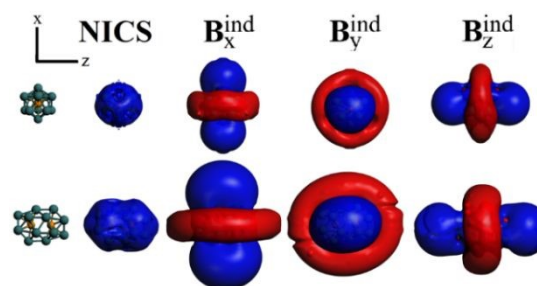
Fig. 7. Magnetic response properties of [\text{Pd}_2@\text{Sn}_{18}]^{4-} , denoting the NICS isosurfaces, and from specific orientations of the external field ( B_z^{\text{ind}} , B_x^{\text{ind}} , and B_y^{\text{ind}} ). Isosurfaces set to \pm 3 ppm, blue - shielding; red - deshielding. Reprinted with permission from Ref. 209 . Copyright Royal Society of Chemistry, 2024.
