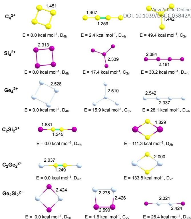
Fig. 2 Optimized geometries of most stable M_2A_2^{2+} clusters of group 14 computed with the PBE/TZ2P method. Bond lengths in Å and CCSD(T)/6-311G*//PBE/TZ2P relative energies in kcal mol -1 . Reprinted with permission from ref. 107 . Copyright Royal Society of Chemistry, 2016.
