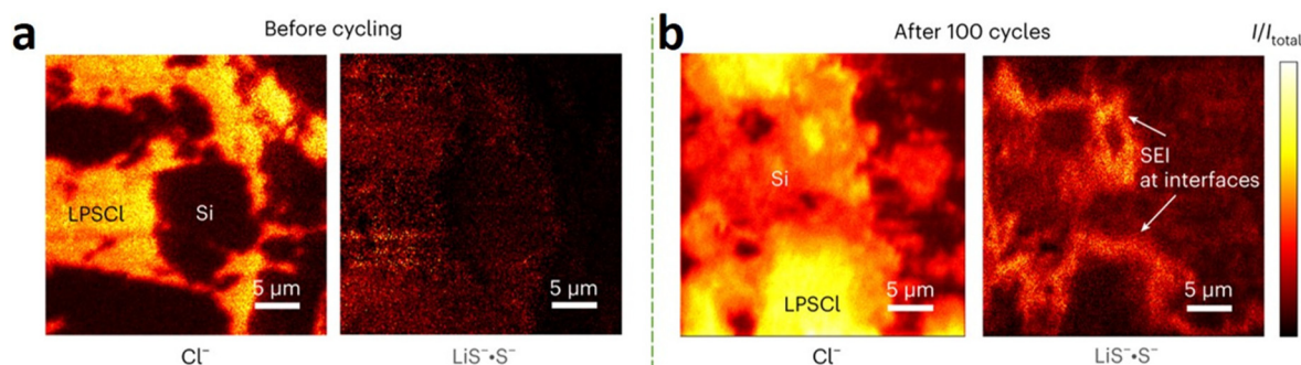
Fig. 32 ToF-SIMS images of the \text{Cl}^- fracture and the product of the \text{Li}^+ and \text{S}^{2-} fractures in \text{Si}/\text{Li}_6\text{PS}_5\text{Cl} composites before cycling (a) and after 100 cycles (b). 362
