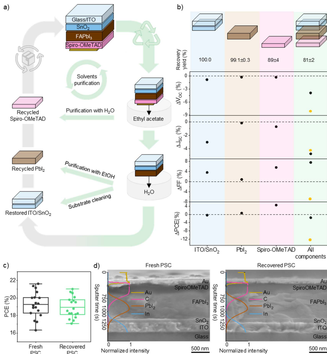
Fig. 1 (a) Schematic illustration of the recovery processes for three critical components of PSCs, i.e. SnO 2 -coated ITO substrates, PbI 2 and Spiro-OMeTAD. Recycling/restoration processes are identified by green arrows, while re-fabrication processes are identified by gray arrows. (b) Photovoltaic parameters percentage variation of recovered samples with respect to fresh samples for single-component and all-component recycling/restoration processes. Recycling yield, calculated as percentage of mass recovered, is reported for single-component and all-component recycling/restoration processes. Yellow dots highlight the variation of PV parameters after the third recovery cycle of all components. (c) Power conversion efficiency box chart for PSCs fabricated with fresh components ("Fresh PSC") and restored ITO/SnO 2 , recycled PbI 2 and Spiro-OMeTAD, simultaneously ("Recovered PSC"). Sample size is 18. Whiskers limit the 1.5 interquartile range, the box identifies the 25th and 75th percentile and the horizontal line represents the average value. (d) SEM cross-sectional images of PSCs fabricated by employing fresh components and, simultaneously, restored ITO/SnO 2 and recycled PbI 2 and Spiro-OMeTAD. ToF-SIMS curves for Au, C, PbI 2 and In are superimposed on SEM images.
