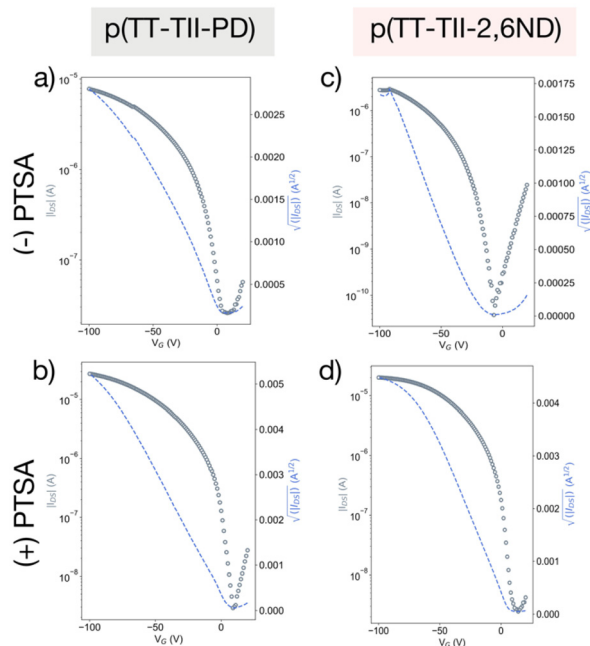
Fig. 4 Typical transfer curves of pristine (−)PTSA and protonated (+)PTSA thin films: (a) pristine p(TT-TII-PD), (b) protonated p(TT-TII-PD), (c) pristine p(TT-TII-2,6ND), and (d) protonated p(TT-TII-2,6ND).
