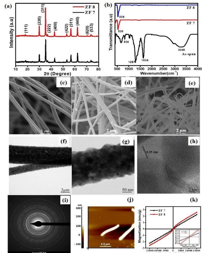
Fig. 1: (a) XRD patterns and (b) FTIR spectra of the samples. SEM micrographs of ZnFe 2 O 4 fibers: (c) as-spun, (d) ZF7, and (e) ZF8. (f-h) TEM micrographs and (i) SAED pattern of the ZF8 sample. (j) AFM topography of ZF8 sample. (k) M-H loops of ZF7 and ZF8 samples.
