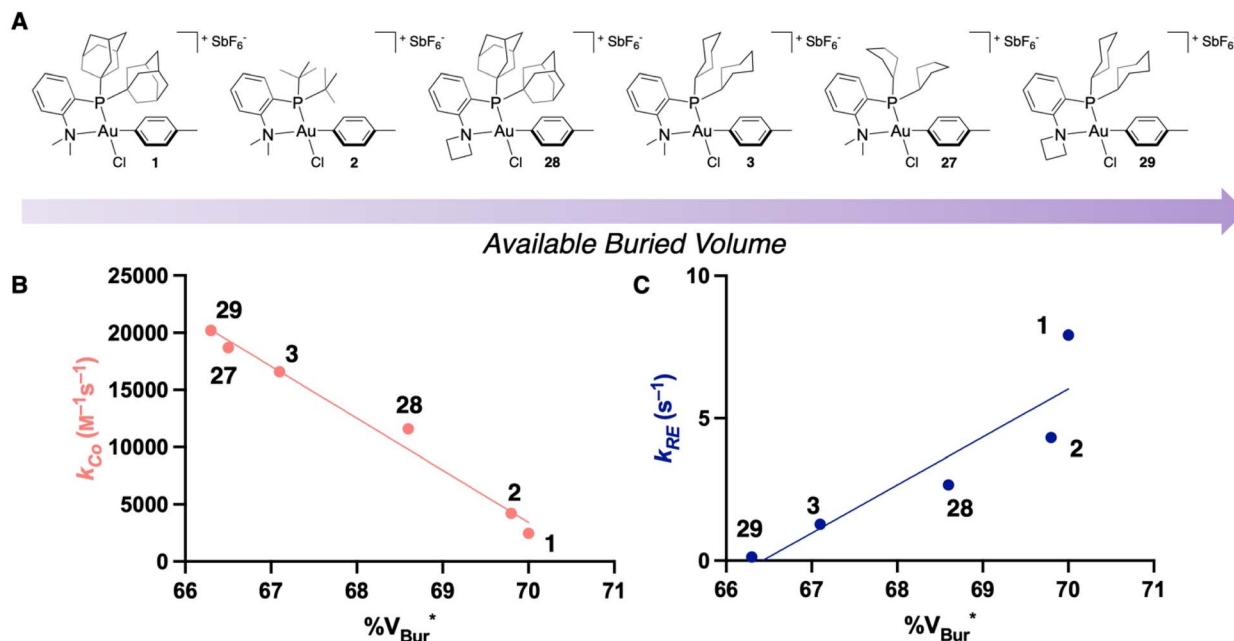
Fig. 8 (A) Ordering of the experimentally characterized Au(III) OACs from this and previous studies in order of least to most available % V Bur . 35 (B) Plot of experimentally determined k_{CO} against % V Bur for the Au(III) OACs shown in Fig. 8A. % V Bur is for the phenyl OAC and the counterion is not included. (C) Plot of experimentally determined k_{RE} against % V Bur for the Au(III) OACs shown in Fig. 8A. % V Bur is for the phenyl OAC and the counterion is not included.
