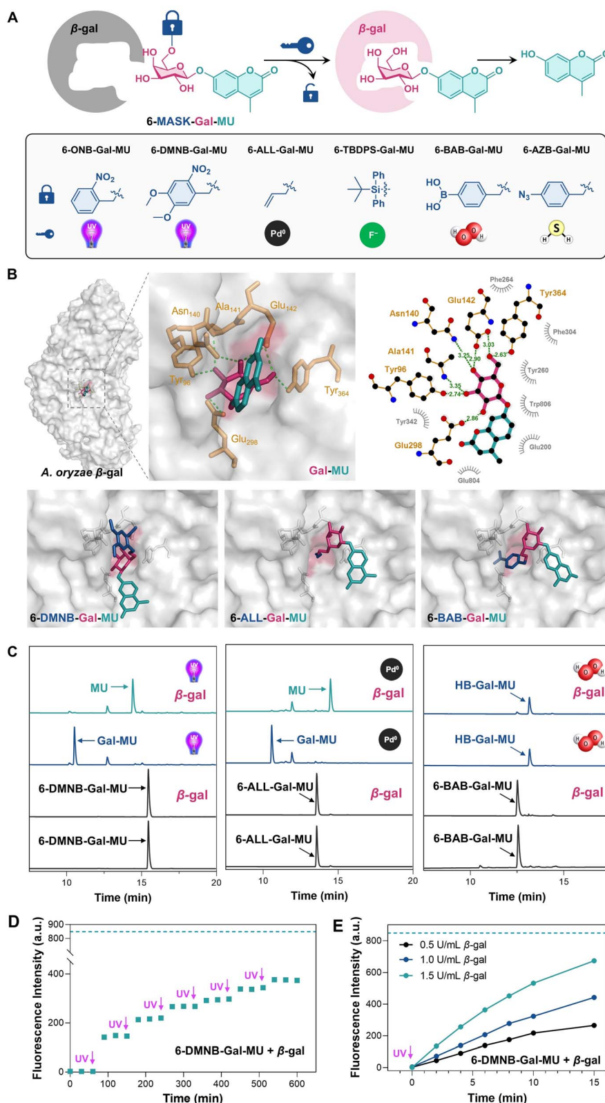
Fig. 1 (A) Design of TACG model compounds, 6-MASK-Gal-MU. (B) The docking of Gal-MU and representative TACG model compounds with A. oryzae β-gal (PDB: 4IUG). β-Gal is shown as a grey surface, key amino acid residues interacting with the hydroxy groups are shown in yellow, and ligand molecules are shown as stick models with the galactose moiety in red, MU in green, and the masking group in blue. (C) HPLC study of the dual-stimulus responsiveness of TACG model compounds. (D) On-demand release of MU from 6-DMNB-Gal-MU solution containing β-gal under UV irradiation (five seconds each). (E) β-Gal concentration- and time-dependent release of MU from 6-DMNB-Gal-MU after UV irradiation. The green dashed lines in (D) and (E) indicate the theoretical maximum fluorescence intensity corresponding to the complete release of MU from 6-DMNB-Gal-MU.
