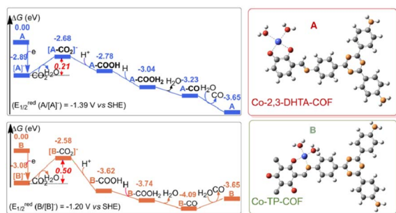
Fig. 6 Gibbs energy profiles of the CO 2 RR-to-CO reaction over Co-2,3-DHTA-COF (A, blue line) and Co-TP-COF (B, orange line). This figure has been reproduced from ref. 65 with permission from American Chemical Society, copyright 2023.
