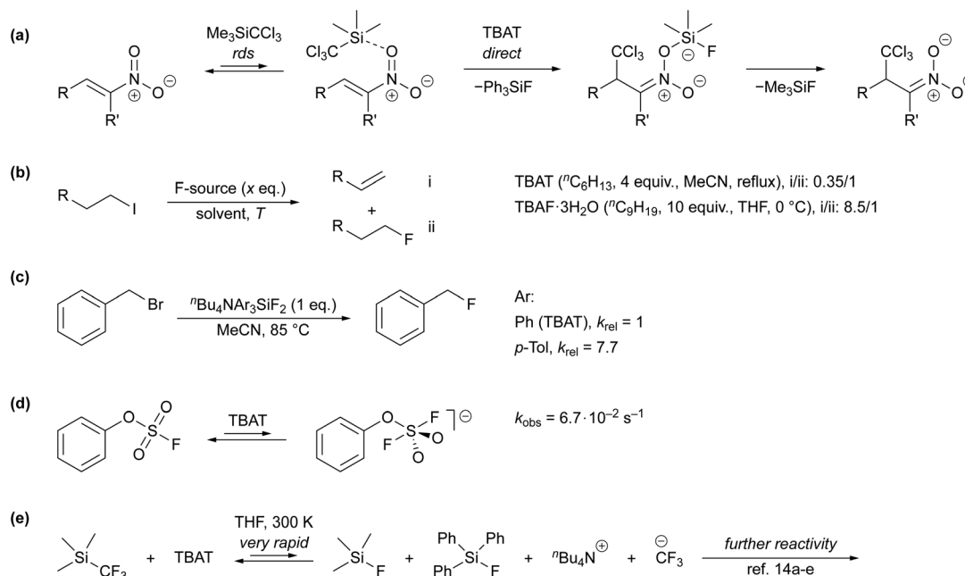
Scheme 1 (a) Mechanistic proposal in a study on the addition of \text{TMSCCl}_3 to nitroalkenes, 10 (b) ratios of \beta -elimination-to-substitution products in reactions of 1-iodoalkanes with TBAT and \text{TBAF} \cdot 3\text{H}_2\text{O} , 1a,11 (c) relative rate constants of fluorination of benzyl bromide using {}^n\text{Bu}_4\text{NAr}_3\text{SiF}_2 , where \text{Ar} = \text{Ph} or p\text{-Tol} , 12 (d) rapid fluoride exchange between TBAT and phenyl fluorosulfate studied via time-dependent saturation transfer NMR spectroscopy, 13 (e) prior mechanistic work on TBAT-initiated reactivity of \text{TMSCF}_3 , where the fluoride transfer from TBAT is very rapid with respect to NMR spectroscopy. In the presence of excess \text{TMSCF}_3 , the \text{CF}_3^- anion(oid) is transient, undergoing rapidly-reversible exergonic equilibrium with [\text{TMS}(\text{CF}_3)_2]^- . 14
