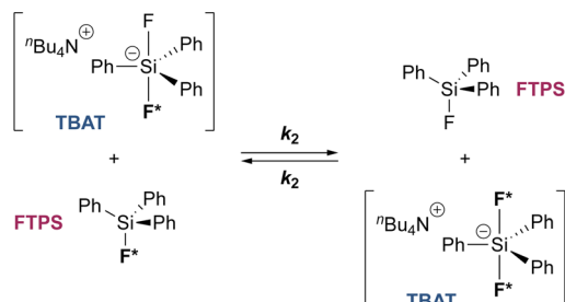
Scheme 2 Two limiting pathways of fluoride transfer from TBAT to FTPS. (a) Dissociative transfer via TBAF, where K_1 = k_1/k_{-1} \ll 1 . (b) Direct bimolecular transfer (the rate constants in each direction, k_2 , are identical, as \Delta G^\circ = 0 ). In each transfer pathway, examples of exchanging fluorine atoms are marked in bold with an asterisk.
