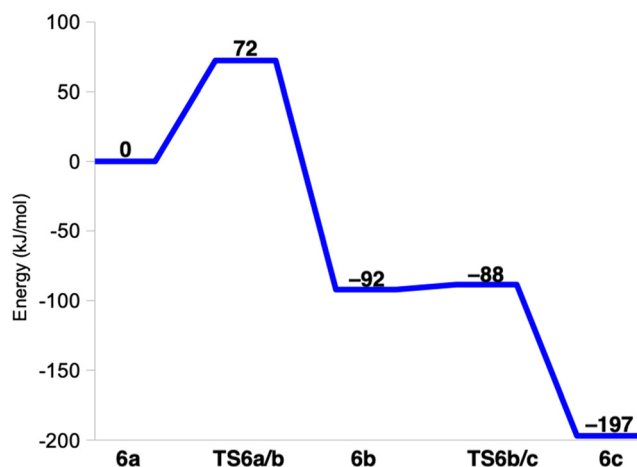
Fig. 7 Energy profile ( \text{kJ mol}^{-1} ) for the reactions involving 6a, 6b and 6c.
