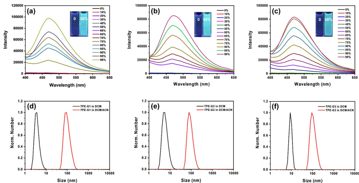
Fig. 3 AIE behaviors of the AIEgen-branched rotaxane dendrimers TPE-Gn ( n = 1, 2 , and 3 ). Fluorescence spectra of TPE-G1 (a), TPE-G2 (b), and TPE-G3 (c) in DCM/ACN with various ACN fractions ( [\text{TPE units}] = 50 \mu\text{M} , \lambda_{\text{ex}} = 345 \text{ nm} ), inset: photographs of TPE-Gn ( n = 1, 2 , and 3 ) in DCM/ACN with 0% (left) and 98% (right) ACN fractions upon UV excitation ( \lambda_{\text{ex}} = 365 \text{ nm} ); DLS data for TPE-G1 (d), TPE-G2 (e), and TPE-G3 (f) in DCM and aggregate states.
