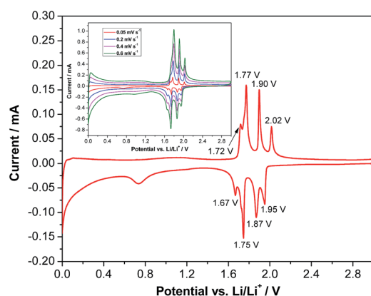
Fig. 2 Cyclic voltammogram of LVP anodes recorded at a scan rate of 0.05 \text{ mV s}^{-1} in the potential range of 3.0–0.0 V vs. \text{Li/Li}^+ . Inset: CV at different scan rates.
