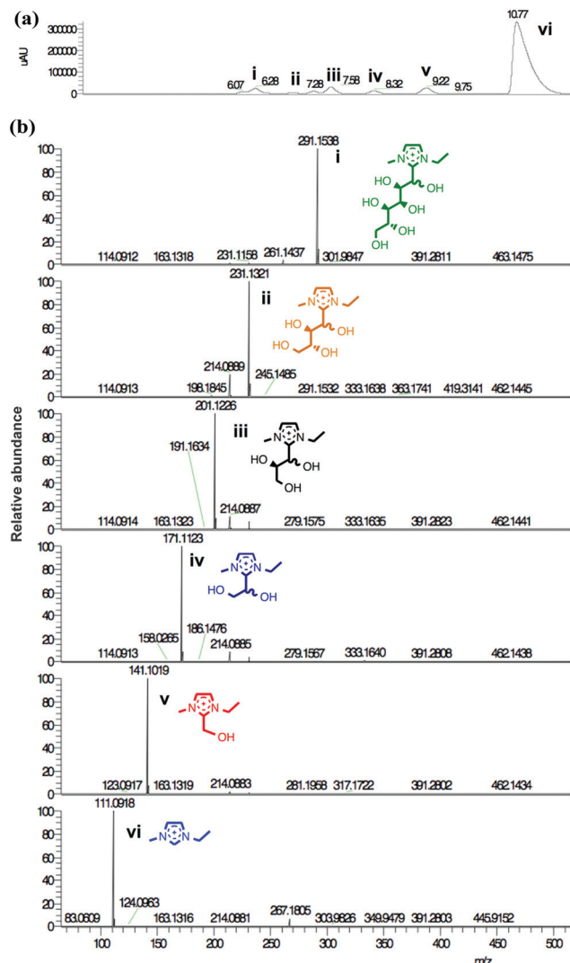
Fig. 4 LCMS investigation of adduct species formed from [C 2 C 1 im]-[OAc], 1a + 10 wt% D-(+)-glucose, 12 , heated to 120 °C for one hour ( t 1 ): (a) survey of peaks i–vi; (b) ESI mass spectra of peaks i–vi.
