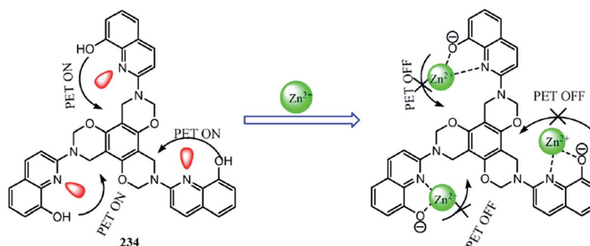
Fig. 198 Chemical structure of receptor 234 and the proposed ligand-zinc complexation mechanism.
