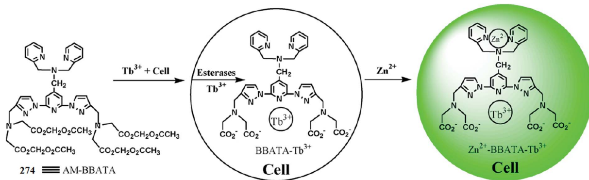
Fig. 238 Schematic of the cell loading and luminescence response of 274- \text{Tb}^{3+} chelate to intracellular \text{Zn}^{2+} ions.
