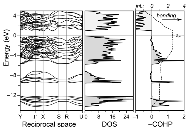
Fig. 2 TB-LMTO-ASA electronic band structure and densities of states (DOS) for Sb 2 Se 3 , and exemplary crystal orbital Hamilton population (COHP) curve for the short Sb(2)–Se(1) contact. The energy integral (“int.”) is given by a dashed line. Negative expectation values of the Hamiltonian reflect stabilisation, and thus we plot –COHP as is convention. 30c The Fermi level \epsilon_F is set as the energy zero.
