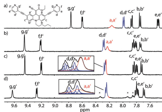
Fig. 4 ^1\text{H} -NMR spectra of (a) ligand L^{\text{Et}} , (b) cage [\text{Pd}_2L^{\text{Et}}_4] at 298 K, (c) the same cage at 333 K and (d) host–guest complex [\text{Pd}_2L^{\text{Et}}_4] containing 1.0 eq. 2,7-naphthyl bisulfonate at 333 K (400 MHz, \text{DMSO}-d_6 ). Cage formation and temperature increase leads to accelerated rotation and sharpening of the a/a' signal (red). Guest uptake slows down spinning of the endohedral rotor, as shown by line fitting analysis of deconvoluted signals d/d' (blue) and a/a' (red). * = signals of the encapsulated guest.
